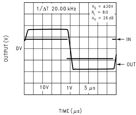
Pulse Response
