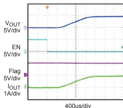
Turn On Delay and Rise Time with 1μF Load I_{OUT}=1A
