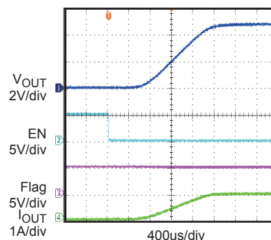
Turn On Delay and Rise Time with 100μF Load I_{OUT}=1A , C_L=100\mu F
