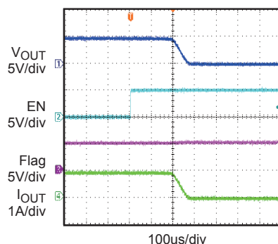
Turn Off Delay and Fall Time with 1μF Load I_{OUT}=1A
