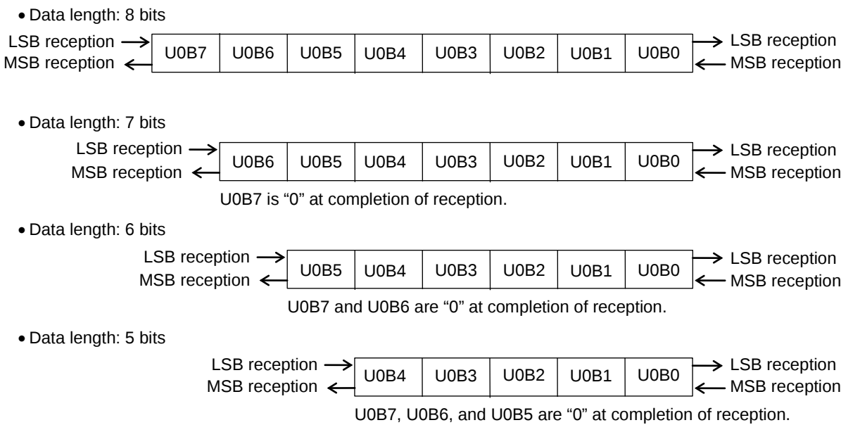
Figure 13-4 Relationship between Transmit/Receive Buffer and Transmit/Receive Data
