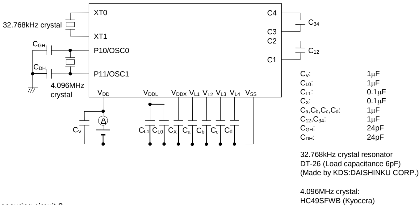
Measuring circuit 2
