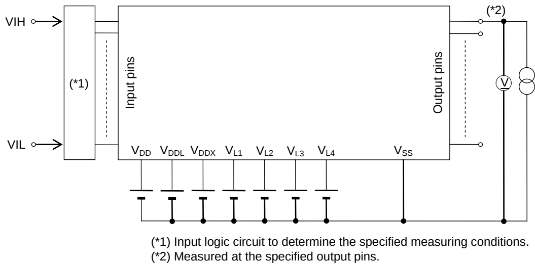
Measuring circuit 2
