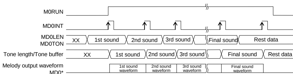
Figure 22-2 Operation Waveform of Melody Driver
