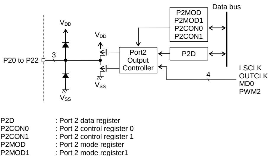
Figure 18-1 Configuration of Port 2
