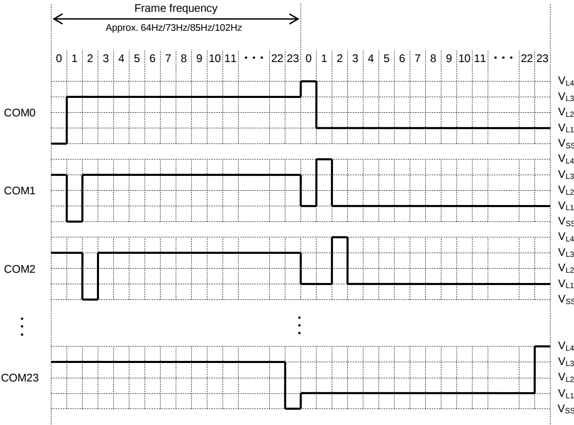
Figure 24-9 (2) Common Output Waveforms for 1/8 Duty and 1/3 Bias
