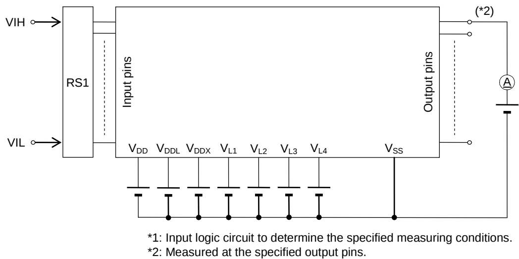
Measuring circuit 4
