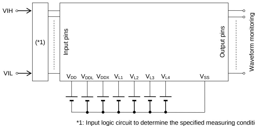
Measuring circuit 5
