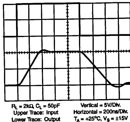
FIGURE 6. VOLTAGE FOLLOWER PULSE RESPONSE
