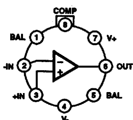
HA-2510/12/15 (TO-99 CAN) TOP VIEW
