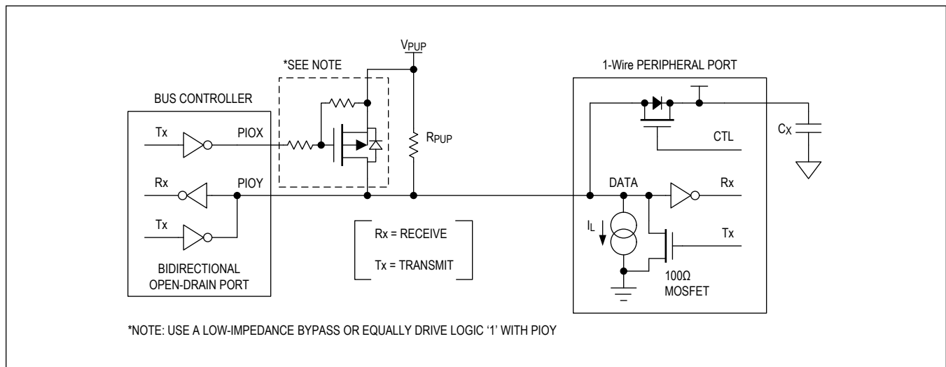
Figure 2. Hardware Configuration
