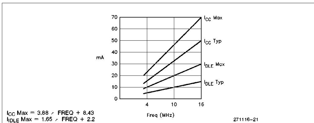
Figure 5. I_{CC} and I_{DLE} vs Frequency
