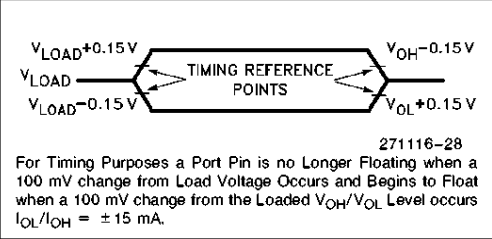
Figure 12. Float Waveforms
