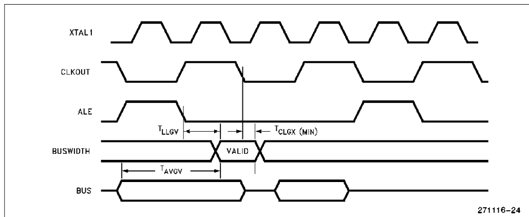
Figure 8. Buswidth Timings
