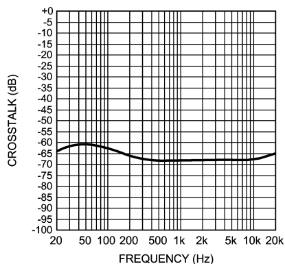
Crosstalk vs Frequency V_{DD} = 3\text{V} , R_L = 16\Omega , P_{OUT} = 42\text{mW} Channel A Driven, Channel B Measured
