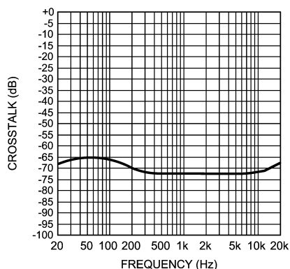
Crosstalk vs Frequency V_{DD} = 2.4\text{V} , R_L = 16\Omega , P_{OUT} = 24\text{mW} Channel A Driven, Channel B Measured
