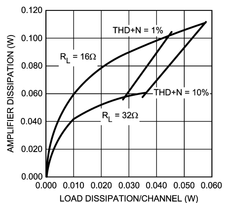
Amplifier Dissipation vs Load Dissipation V_{DD} = 3.0\text{V}
