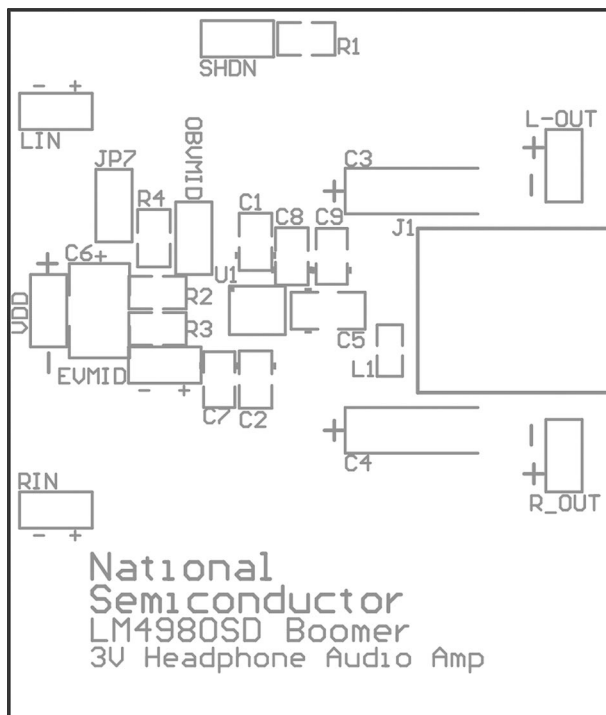
FIGURE 8. Silkscreen Layer
