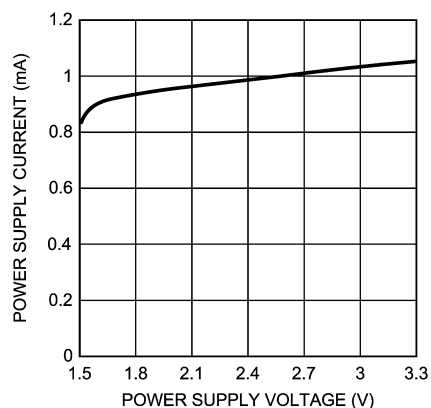
Power Supply Current vs Power Supply Voltage V_{IN} = 0\text{V}
