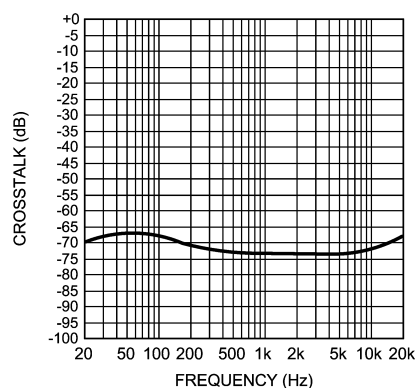
Crosstalk vs Frequency V_{DD} = 1.8\text{V} , R_L = 16\Omega , P_{OUT} = 11\text{mW} Channel B Driven, Channel A Measured
