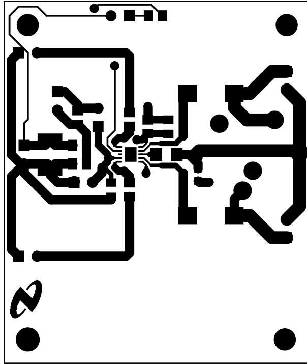
FIGURE 6. Top Layer
