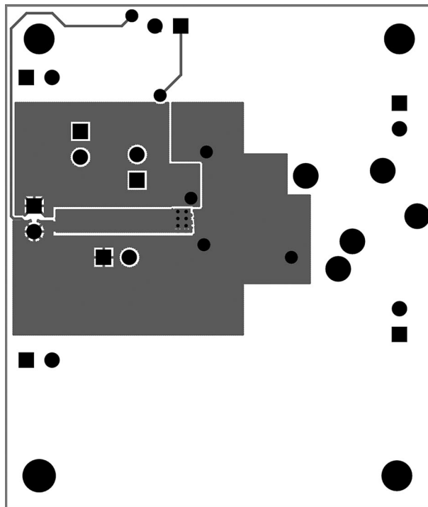
FIGURE 7. Bottom Layer
