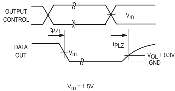
Figure 10. 3-State Output Low Enable and Disable Times
