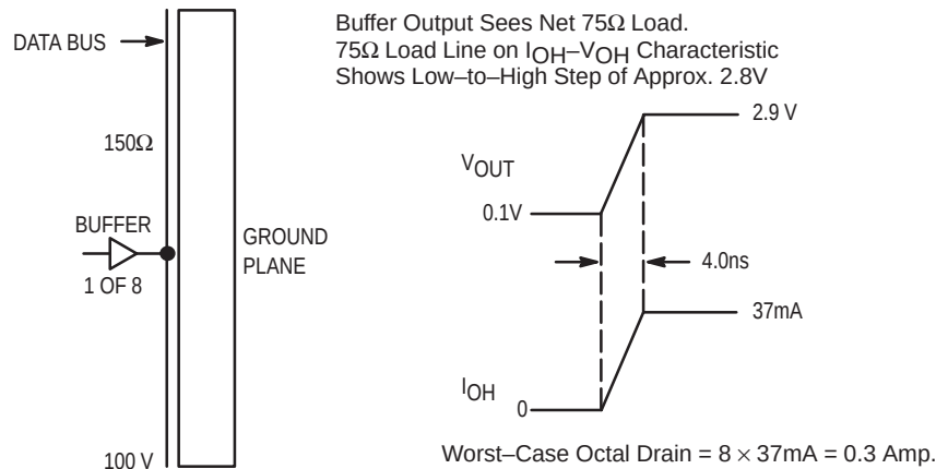
Figure 23. Octal Buffer Driving a 150 \Omega Bus
