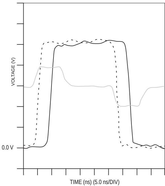
Figure 17. Reverse Crosstalk on PCB Traces
