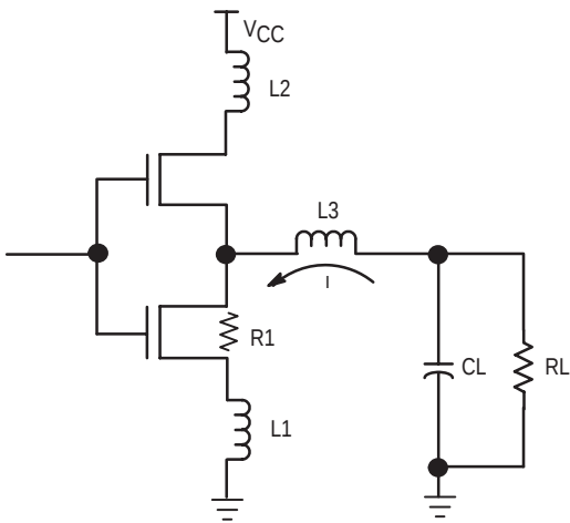
Figure 18. Output Model
