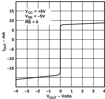
Figure 8. Output Current vs. Voltage
