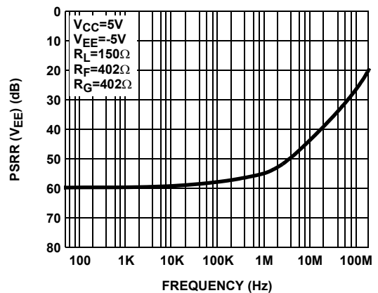
FIGURE 12. PSRR -5V
