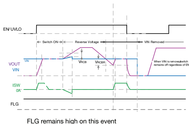
Fig. 40 - Reverse Protection
