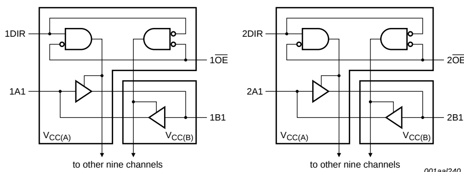
Fig 1. Logic diagram
