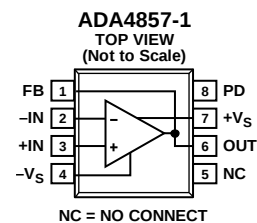
Figure 2. 8-Lead SOIC (R)
