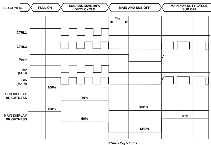
Figure 20. Application Timing
