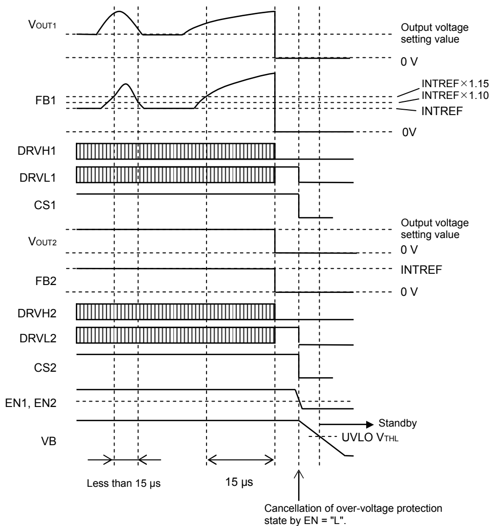
<Timing chart>
