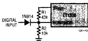
Figure 5. Digital Input Shutdown Level Control
