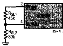
Figure 11a. External Slope Compensation Resistors
