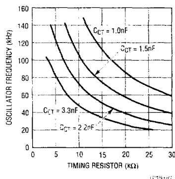
Figure 2. Oscillator Frequency vs R CT , C CT
