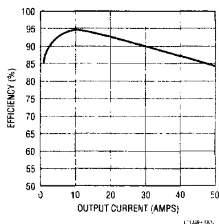
48V to 5V Efficiency Curve
