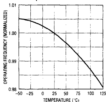
Operating Frequency (Normalized) vs Temperature
