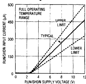
Run/Shutdown Input Current vs Pin Voltage
