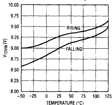
UVLO Thresholds vs Temperature
