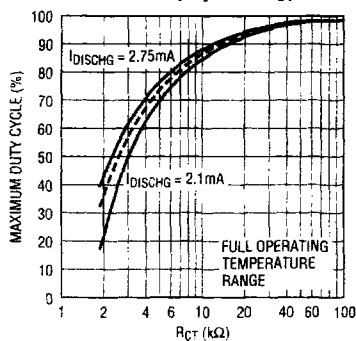
Maximum Duty Cycle vs RCT
