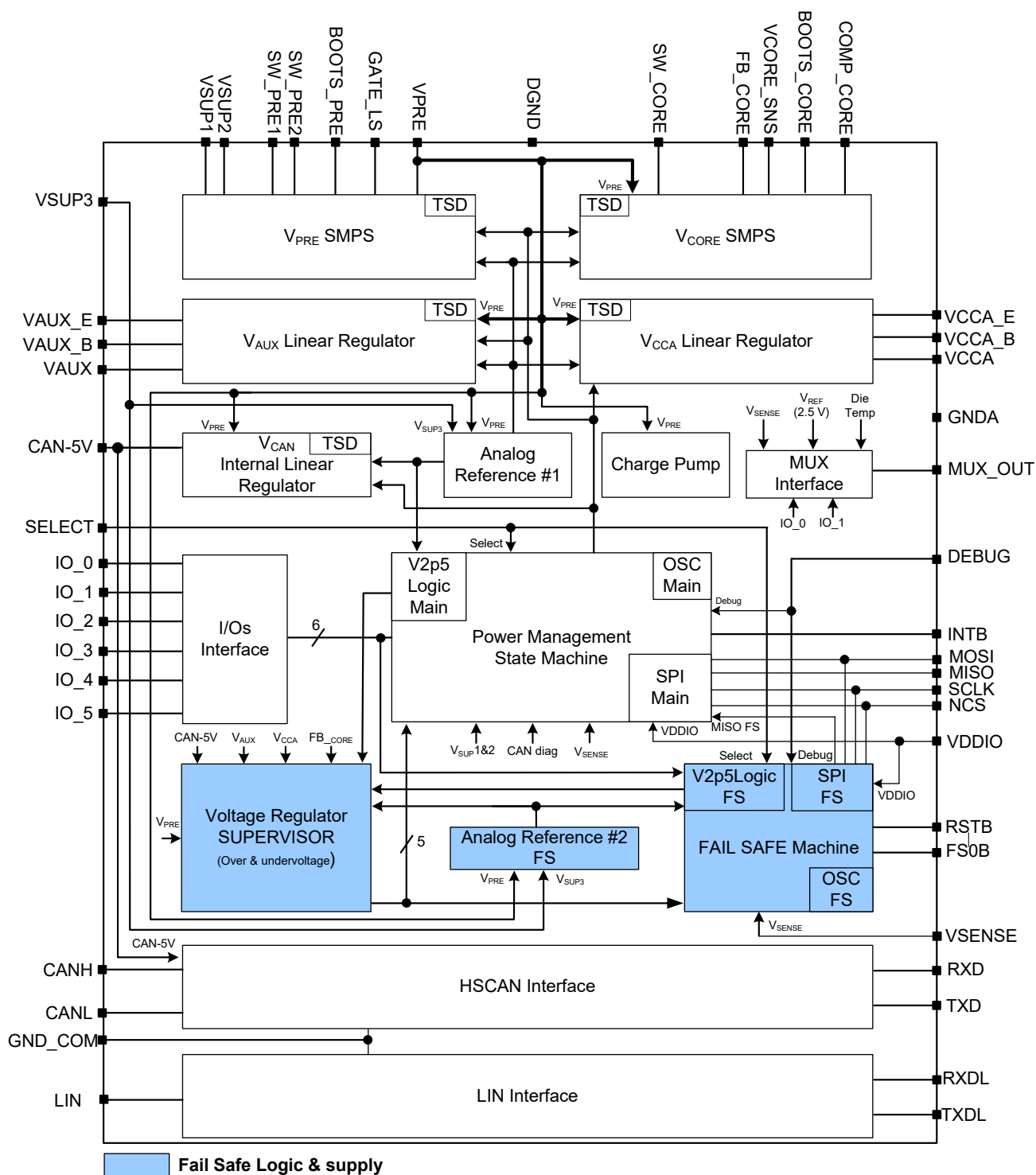
Figure 3. 33907L/33908L with CAN and LIN simplified internal block diagram
