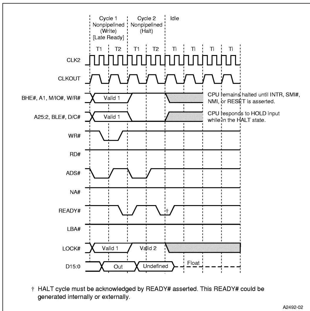
Figure 26. Halt Cycle
