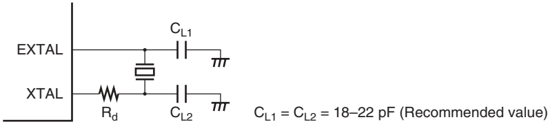
Figure 4.2 Connection of the Crystal Resonator (Example)
