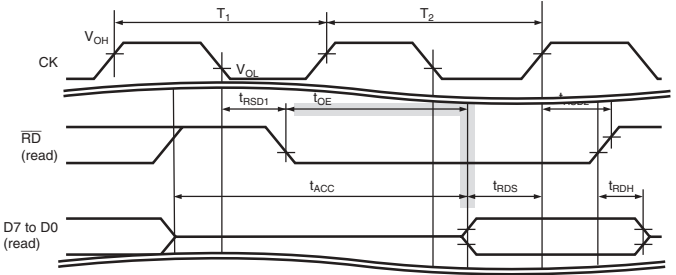
Figure 25.10 Basic Cycle (No Waits)
