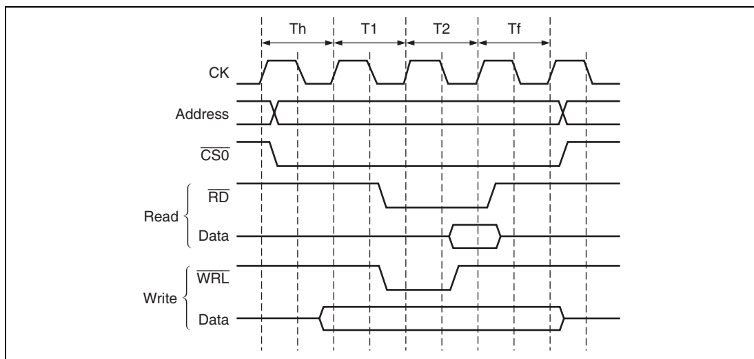
Figure 9.6 \overline{\text{CS}} Assert Period Extension Function
