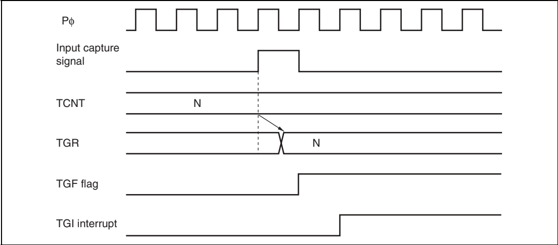
Figure 10.65 TGI Interrupt Timing (Input Capture)
