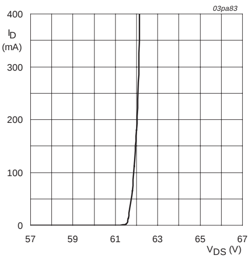
Fig 16. Overvoltage clamping characteristic; drain current as a function of drain-source voltage; typical values.
