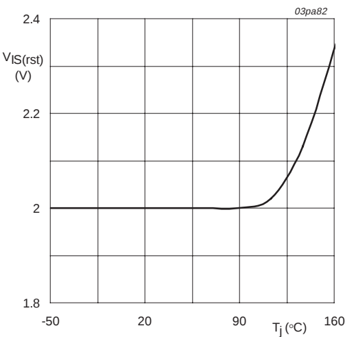
Fig 15. Input-source reset voltage as a function of junction temperature; typical values.
