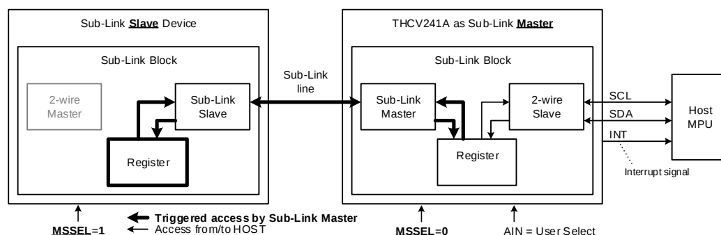
Figure 16. Host MPU to Sub-Link Slave Register via THCV241A access configuration
