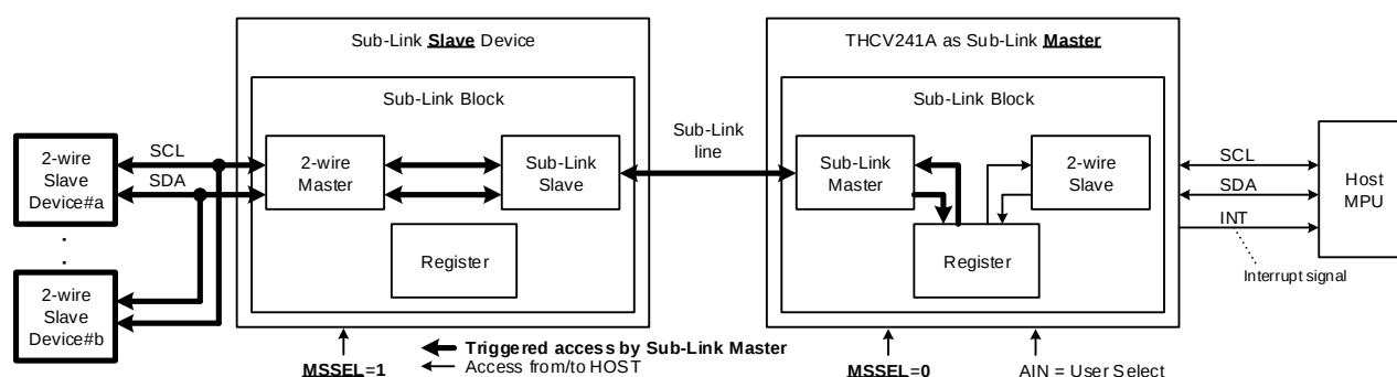
Figure 17. Host MPU to 2-wire slave devices connected to Sub-Link Slave via THCV241A access configuration
