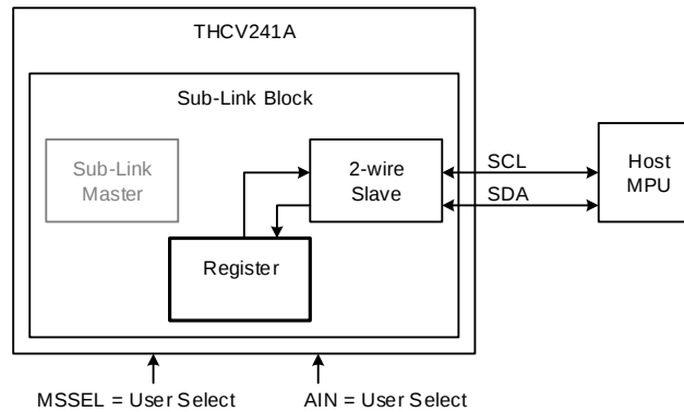
Figure 13. Host to THCV241A local register access configuration
