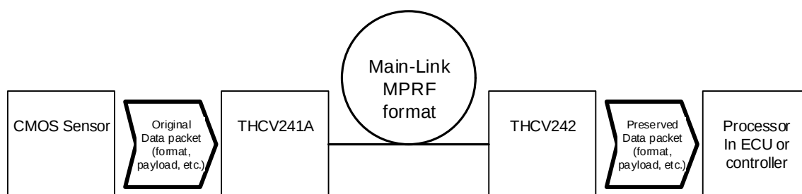
Figure 4. MPRF (Main-Link PRivate Format)
