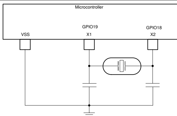
Figure 7-13. External Crystal
