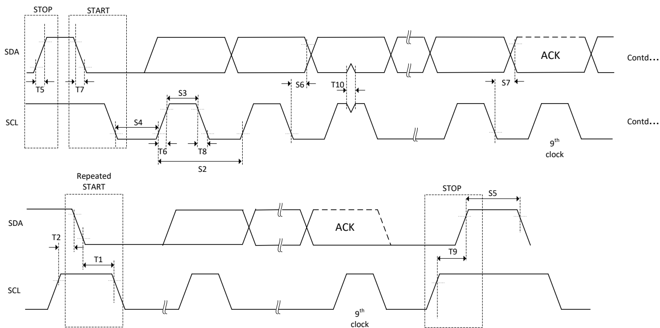
Figure 7-54. I2C Timing Diagram
