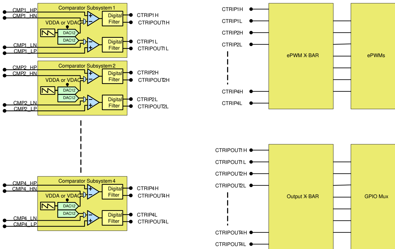
Figure 7-36. CMPSS Connectivity
