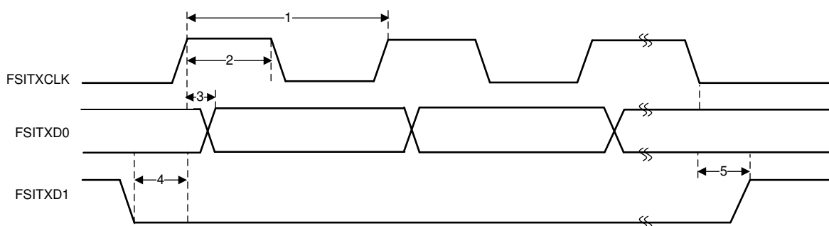
Figure 7-69. FSITX SPI Signaling Mode Timings
