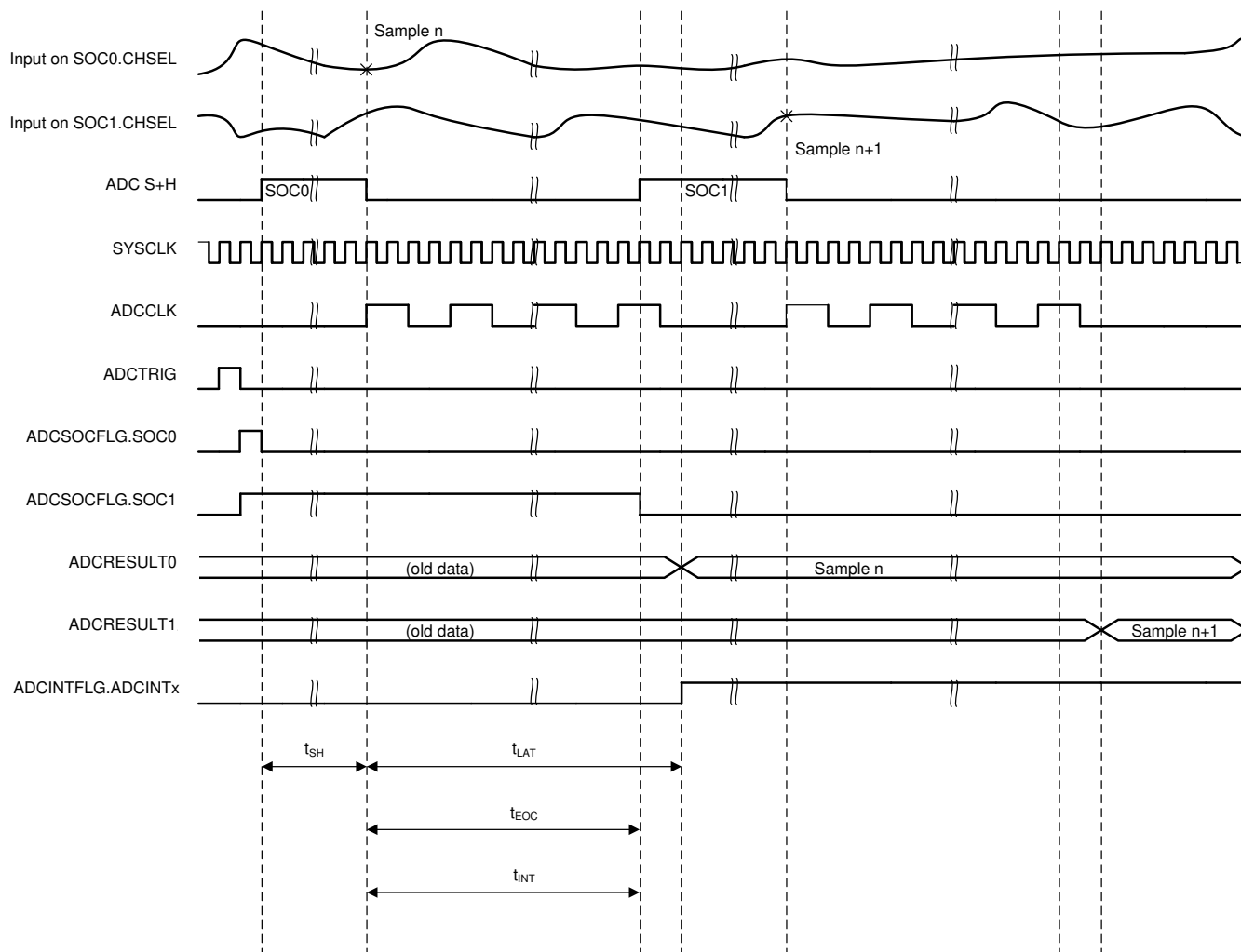
Figure 7-35. ADC Timings
