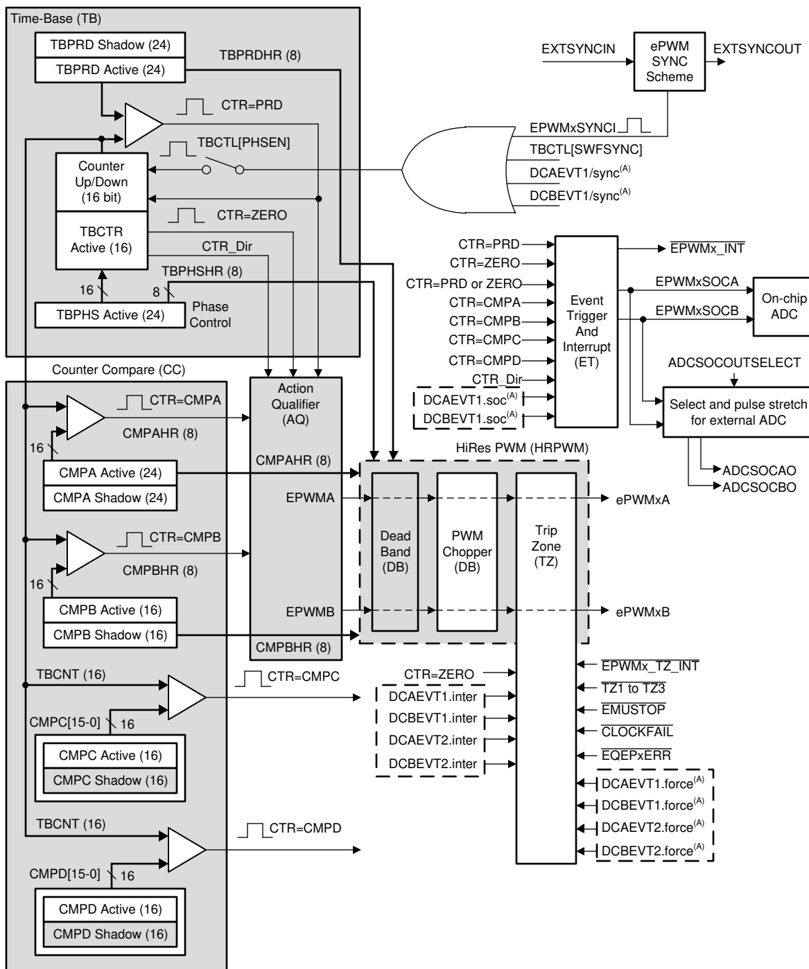
Figure 7-42. ePWM Submodules and Critical Internal Signal Interconnects
