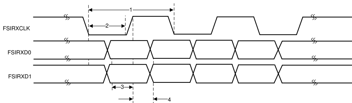
Figure 7-68. FSIRX Timings
