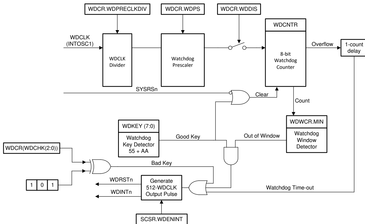
Figure 8-3. Windowed Watchdog
