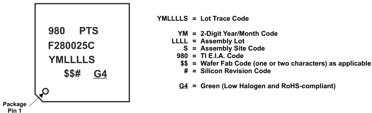
Figure 10-3. Package Symbolization for PT Package
