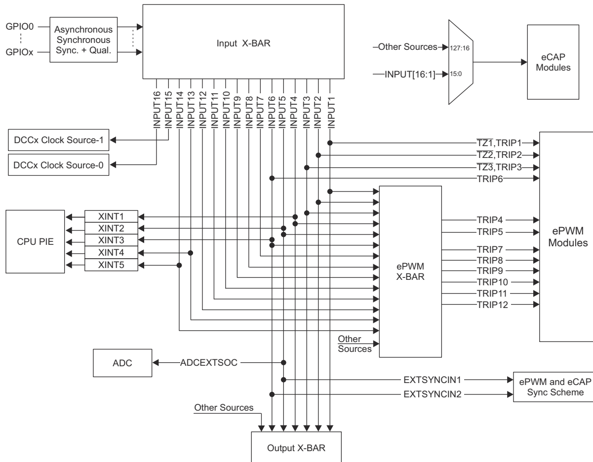
Figure 6-4. Input X-BAR
