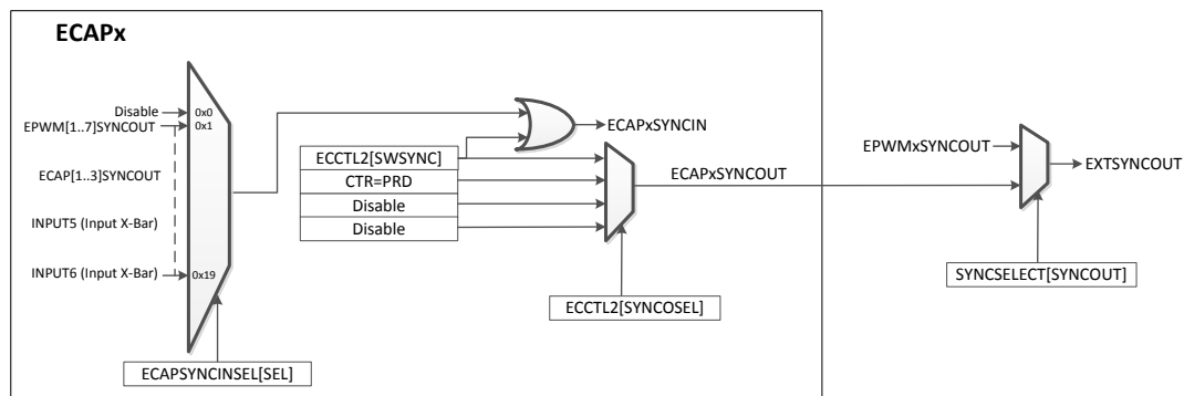
Figure 7-48. eCAPSynchronization Scheme
