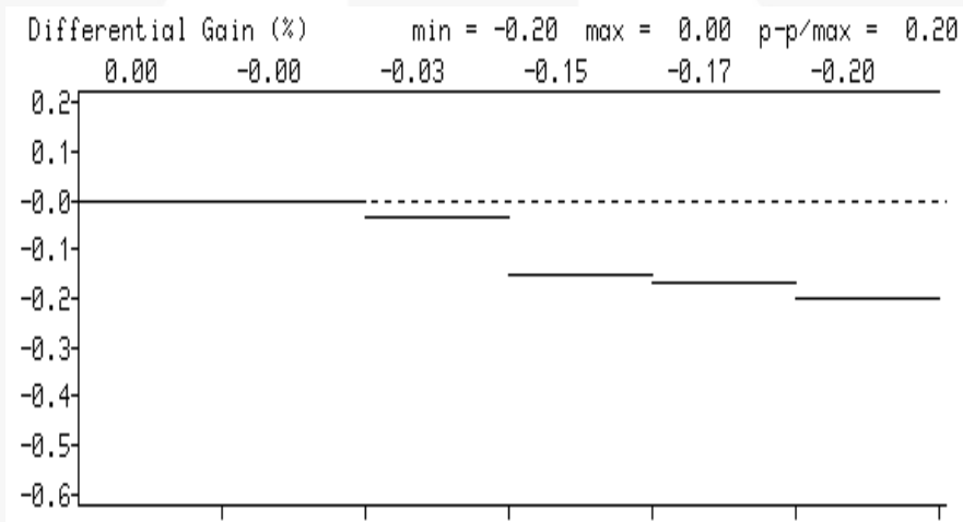
Figure 7. Differential Gain
