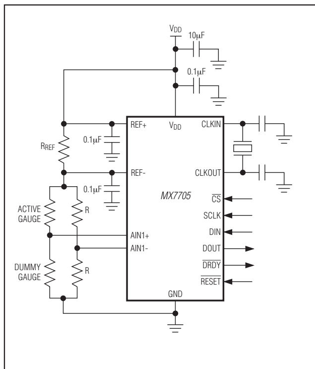
Figure 12. Strain-Gauge Measurement
