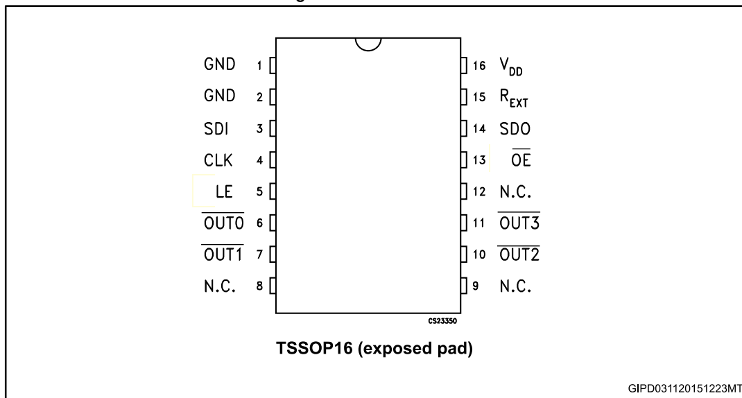
Figure 2: Pin connection
