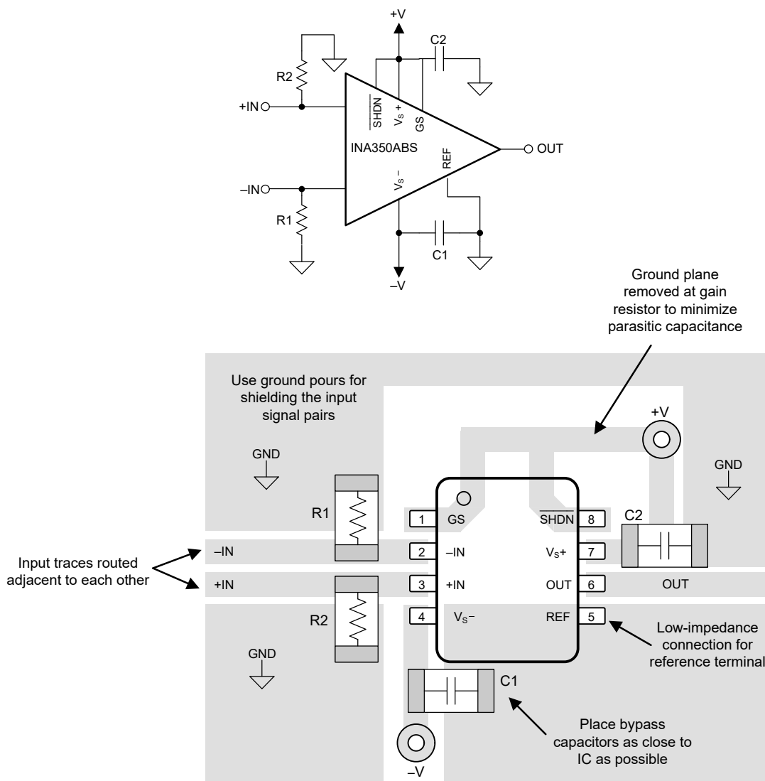
Figure 9-6. Example Schematic and Associated PCB Layout
