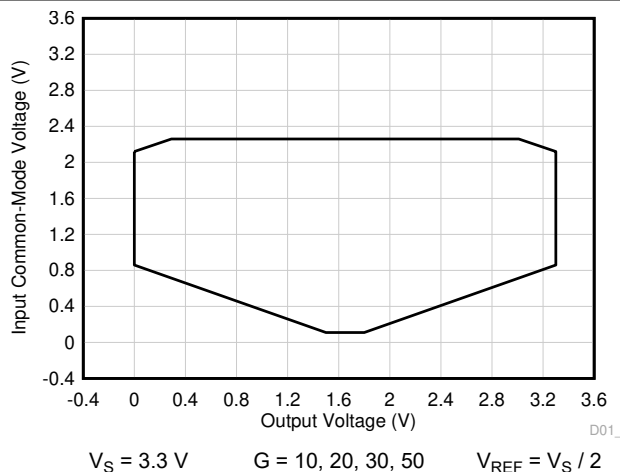
Figure 7-52. Input Common-Mode Voltage vs Output Voltage (High CMRR Region)
