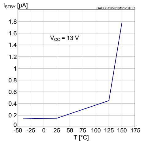
Figure 15. Standby current
