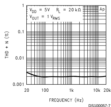
Equalizer Output THD+N vs Frequency
