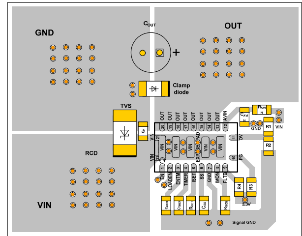
Figure 10: Recommended Layout
