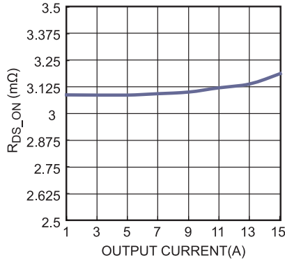
R DS_ON vs. Load Current V_{IN}=12V
