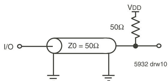
Figure 6. Output Load
