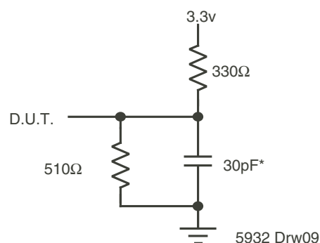
Figure 7. Output Load
