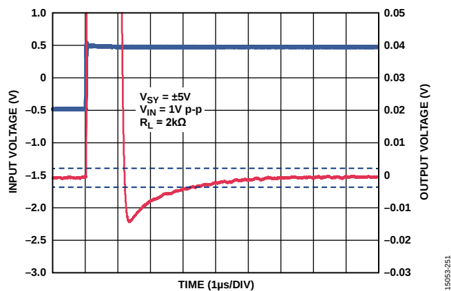
Figure 42. Positive 0.1% Settling Time, V_{SV} = \pm 5\text{ V}
