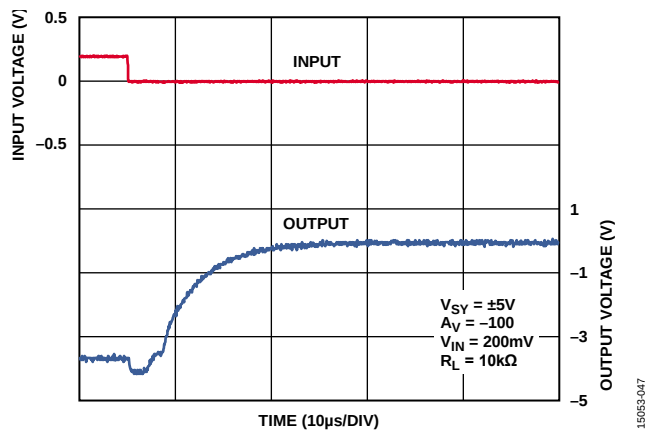
Figure 40. Negative Overload Recovery, V_{SV} = \pm 5\text{ V}
