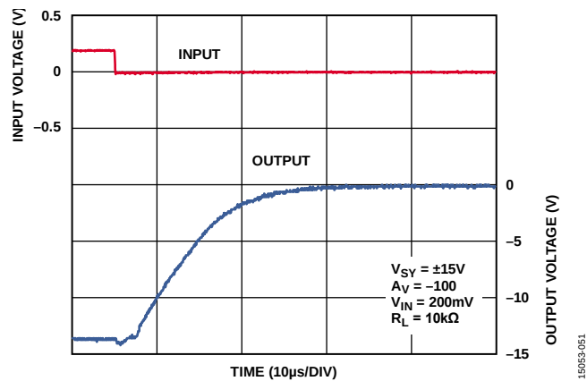
Figure 43. Negative Overload Recovery, V_{SV} = \pm 15\text{ V}
