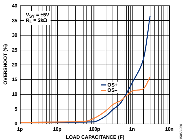
Figure 41. Small Signal Overshoot vs. Load Capacitance, V_{SV} = \pm 5\text{ V}
