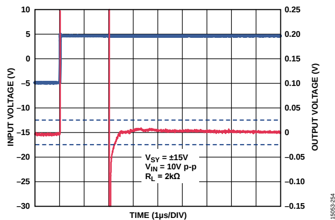
Figure 45. Positive 0.1% Settling Time, V_{SV} = \pm 15\text{ V}
