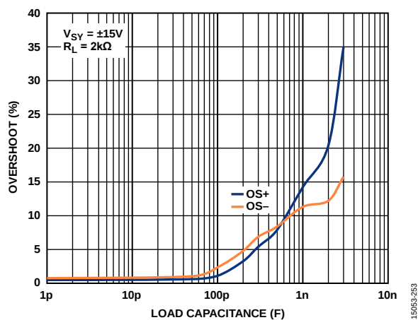
Figure 44. Small Signal Overshoot vs. Load Capacitance, V_{SV} = \pm 15\text{ V}
