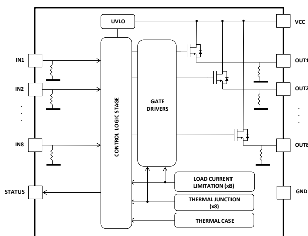
Figure 1. Internal schematic
