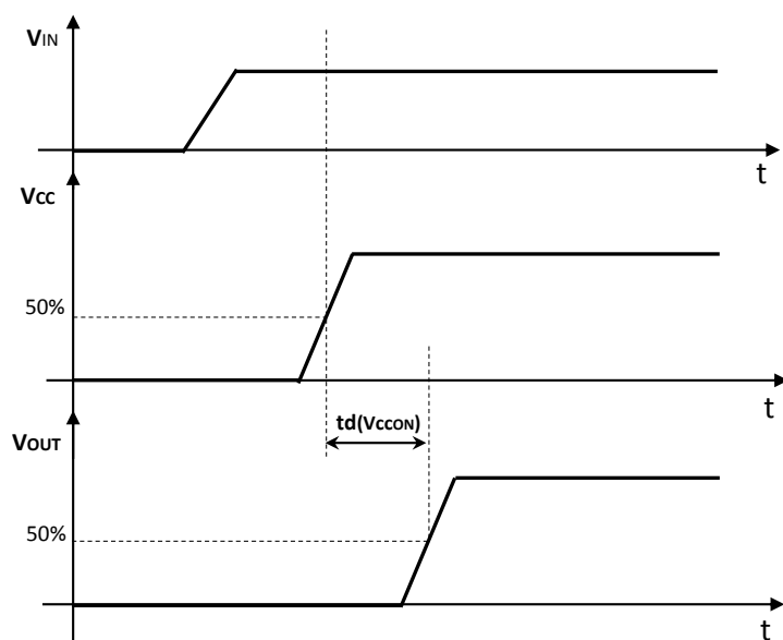
Figure 7. V_{CC} turn-ON
