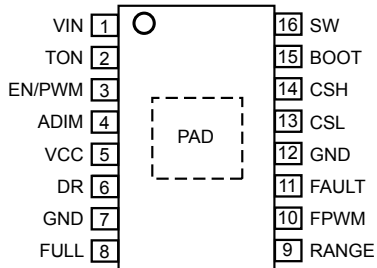
Pinout Diagram for A6216 (LP Package)
