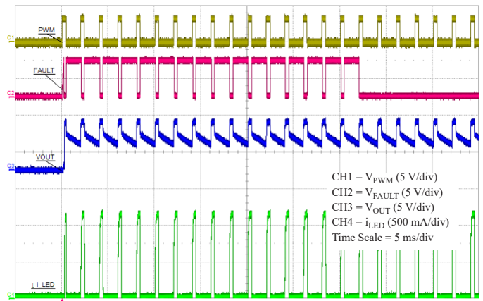
Figure 31: V_{IN} too low for LED regulation. PWM = 500 Hz 20% (400 \mu s). FAULT toggles each time PWM = H, but stays Low after 16 PWM pulses.
