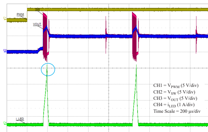
Figure 19: In case of sense resistor short fault – Output current rises until it trips SW OCP at ~3.5 A. The IC shuts off and retries after ~1 ms cooldown period.
