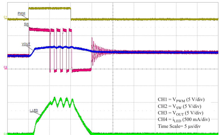
Figure 10: PWM Dimming with on-time of just 10 \mu s – R_{TON} = 442 \text{ k}\Omega , L = 22 \text{ }\mu\text{H} , V_{IN} = 12 \text{ V} , Output = 2 \times LED at 1 A. Note that the LED current takes \sim 5 \mu\text{s} to ramp up to its steady-state value.
