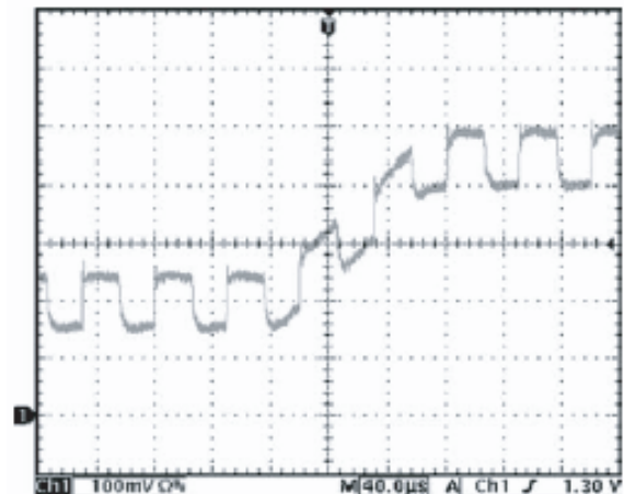
Figure 4. VID On-the-Fly Waveforms, Circuit of Figure 5, VID Change = 5mV, 5 \mu s, 50 steps, Iout Change = 5A to 65A
