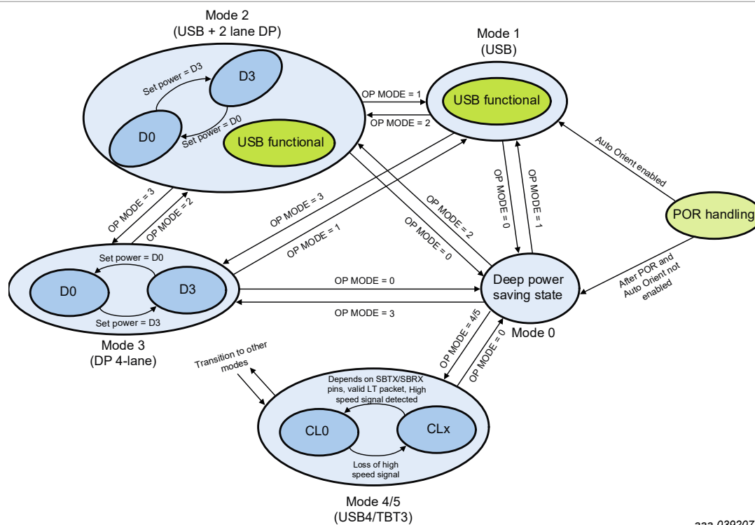
Figure 7. Mode transition state diagram
