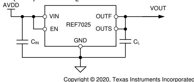
Figure 9-1. Basic Connections
