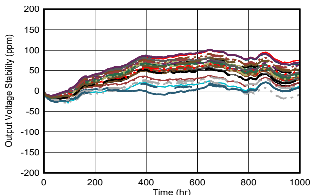
Figure 8-5. Long Term Stability VSSOP
