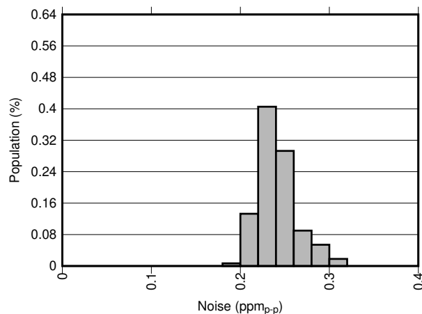
Figure 7-19. 0.1-Hz to 10-Hz Voltage Noise Distribution (300 units)
