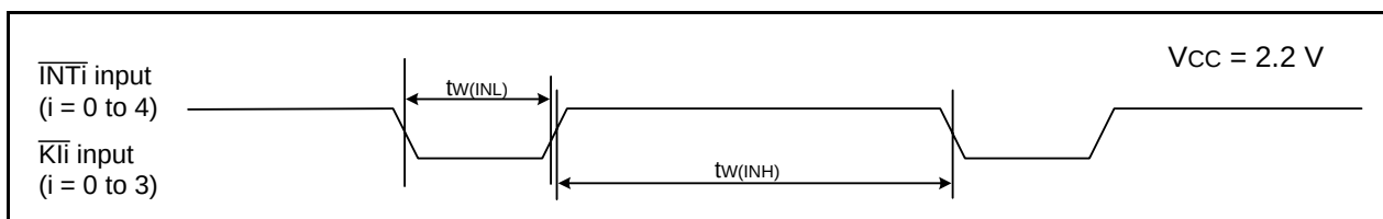
Figure 5.21 Input Timing Diagram for External Interrupt \overline{INTi} and Key Input Interrupt \overline{Kli} when V_{CC} = 2.2 \text{ V}
