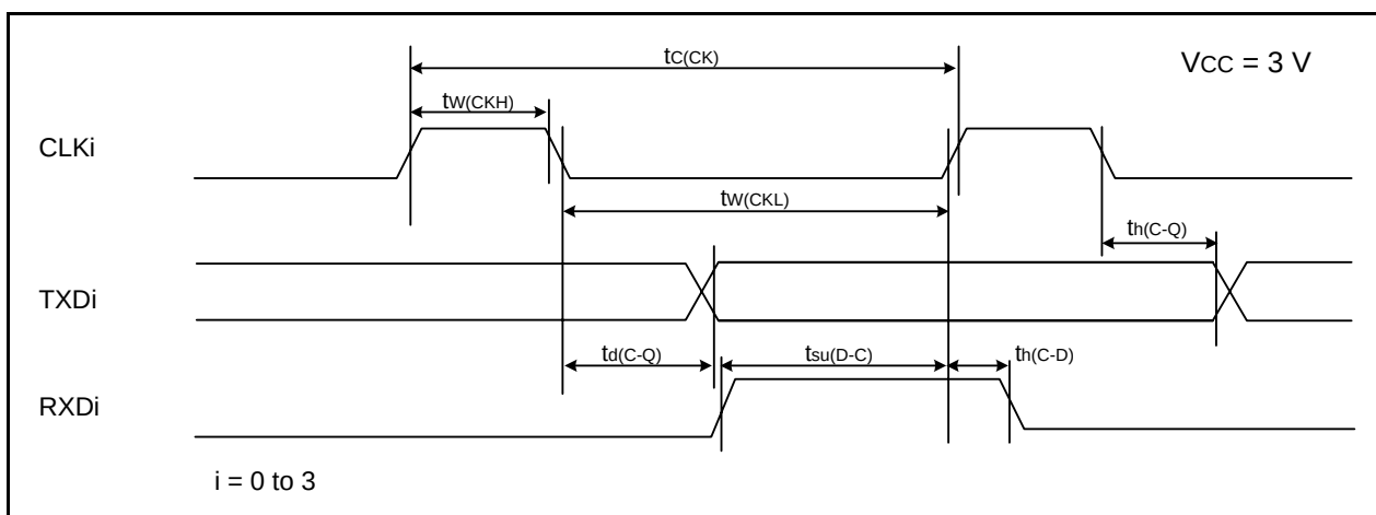
Figure 5.37 Serial Interface Timing Diagram when Vcc = 3 V
