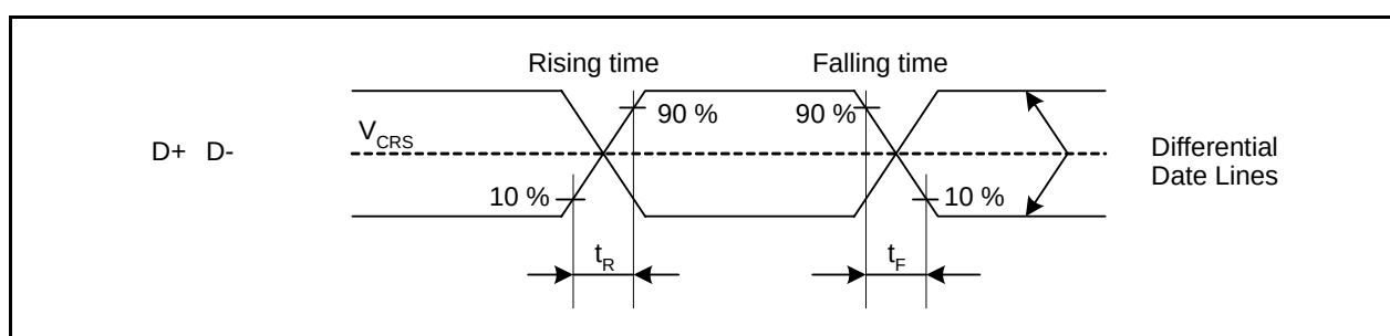
Figure 5.23 Data Signal Timing Diagram
