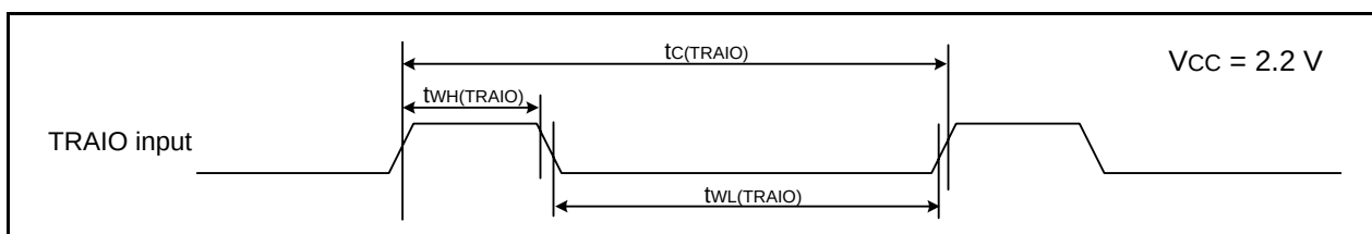
Figure 5.40 TRAIO Input Timing Diagram when V_{CC} = 2.2\text{ V}
