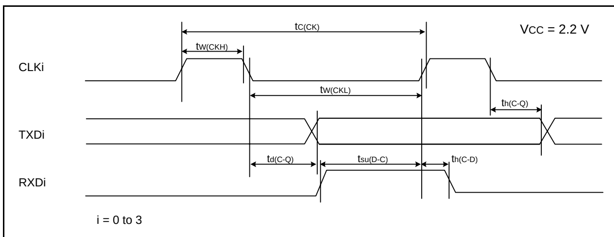
Figure 5.20 Serial Interface Timing Diagram when V_{CC} = 2.2 \text{ V}
