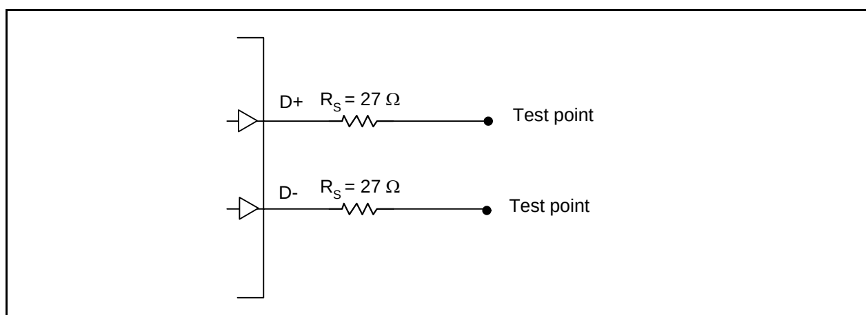
Figure 5.24 Load Condition
