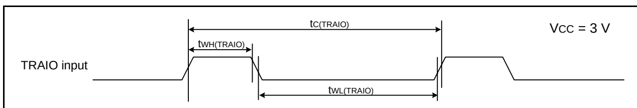
Figure 5.15 TRAIO Input Timing Diagram when V_{CC} = 3\text{ V}
