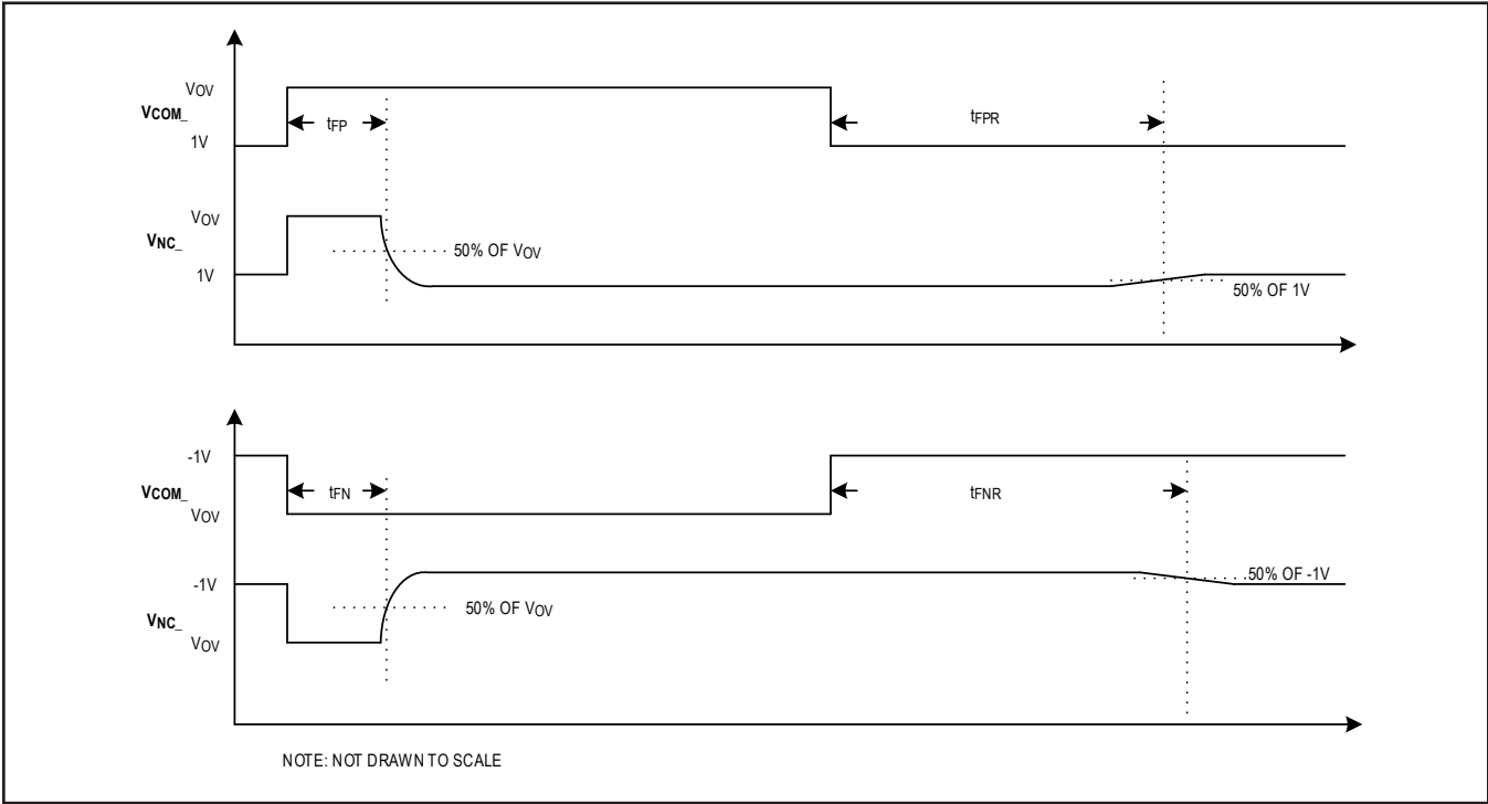
Figure 1. Timing Diagram
