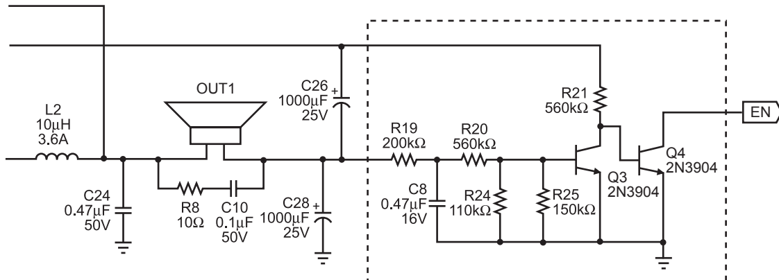
Figure 2—Alternate Configuration for High V_{DD} Applications
