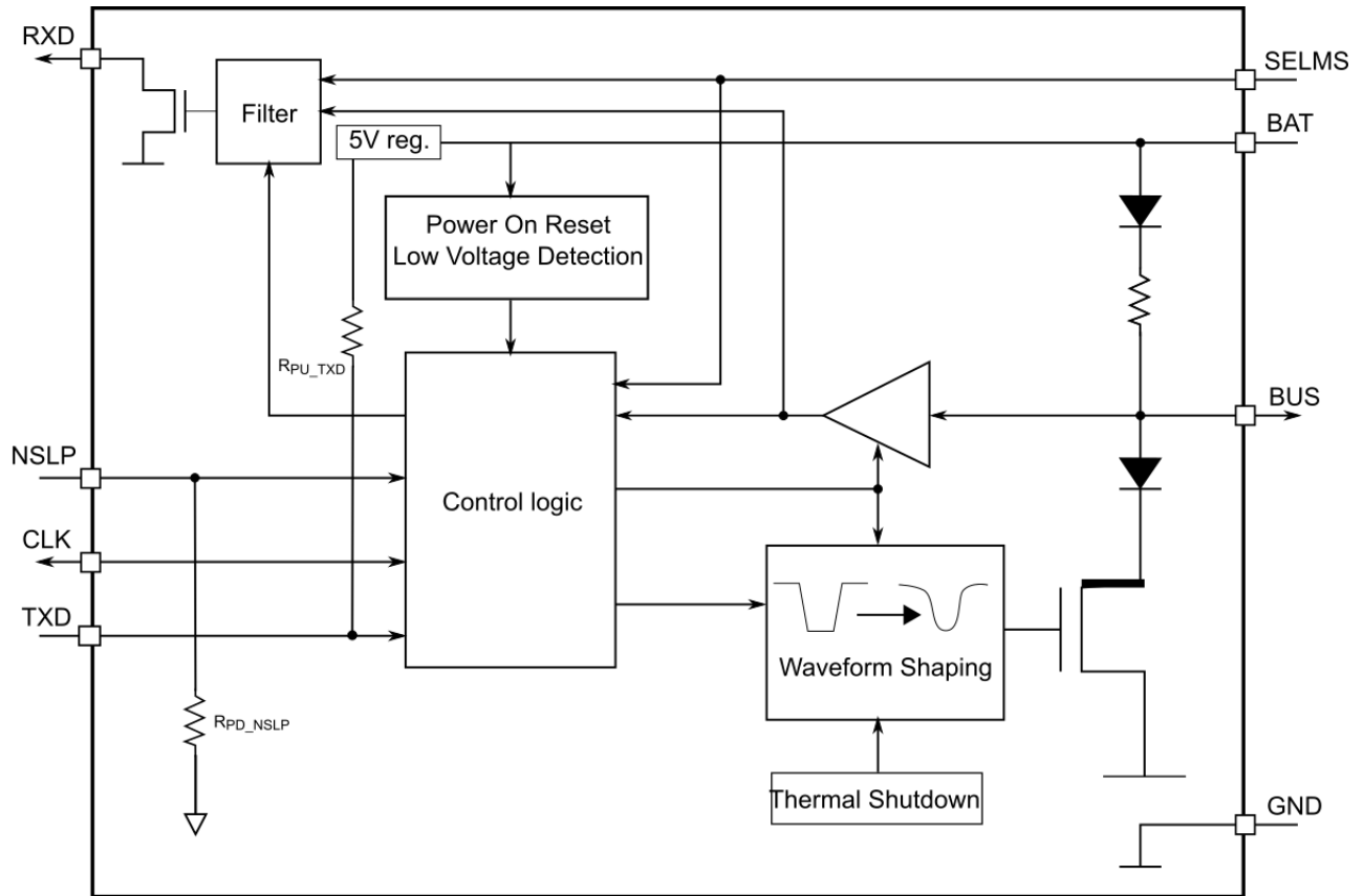
Figure 4-1. Block Diagram
