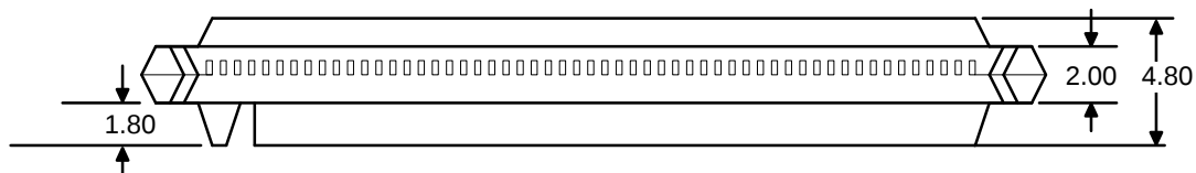
Side View
