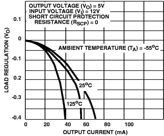
FIGURE 5. LOAD REGULATION WITH CURRENT LIMITING
