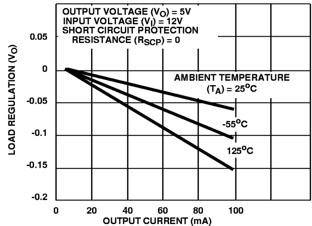
FIGURE 3. LOAD REGULATION WITHOUT CURRENT LIMITING
