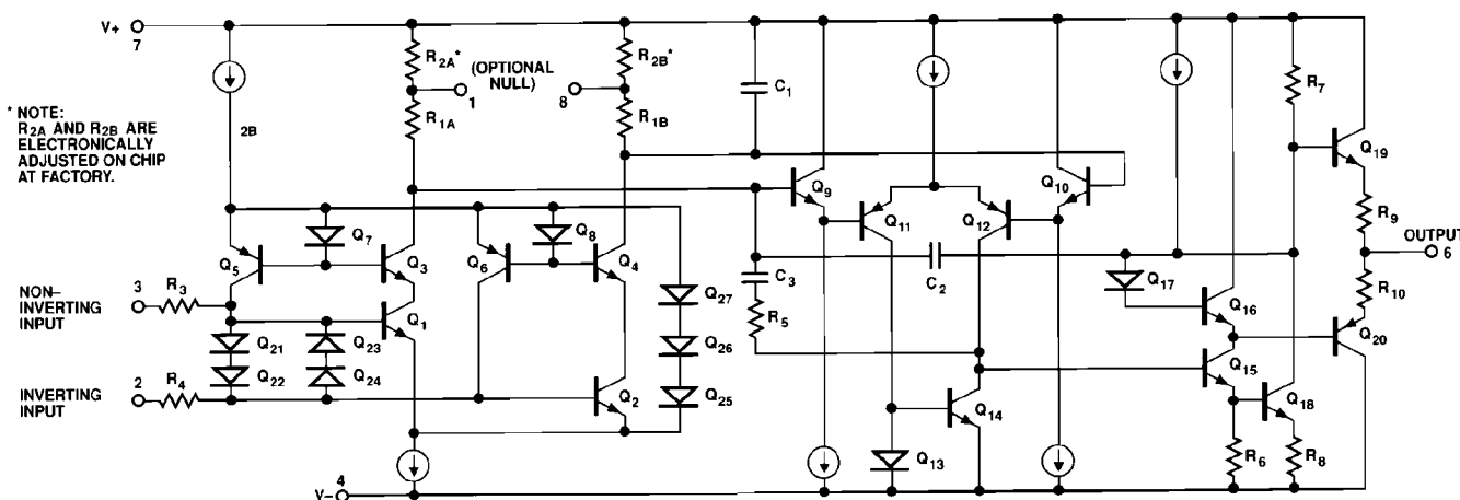
Figure 1. Simplified Schematic
