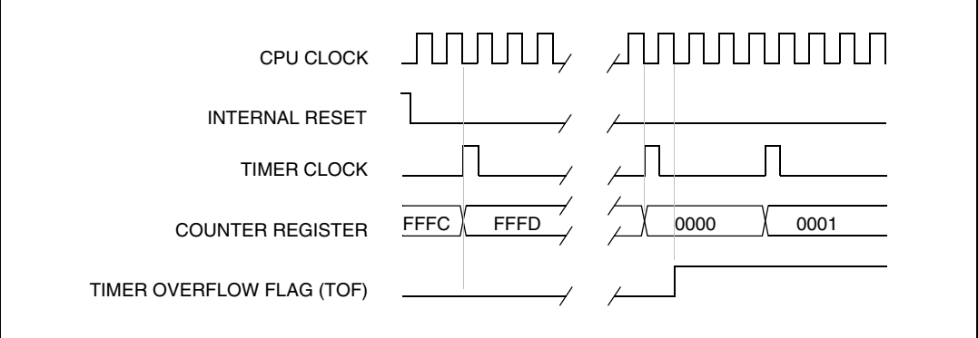
Figure 45. Counter timing diagram, internal clock divided by 4
