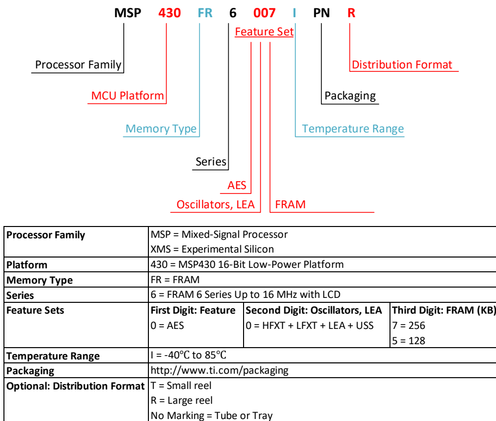
Figure 11-1. Device Nomenclature
