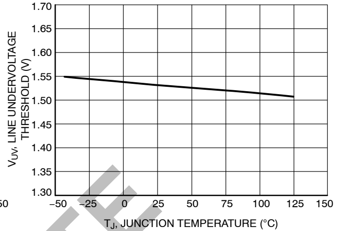
Figure 11. Line Undervoltage Threshold versus Junction Temperature
