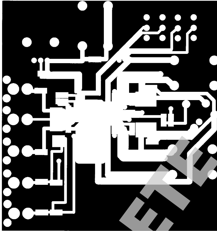
Layer 2 - ( Not to Scale )
