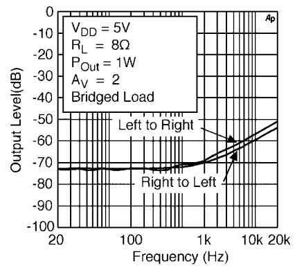
Crosstalk
