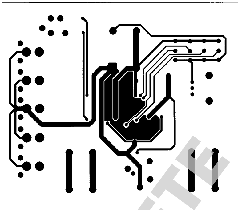
FIGURE 7. Recommended LQ PC Board Layout: Bottom-Side Layout
