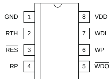
SOIC-8, TSSOP-8, DIL-8 (Top View) D, PW, N or J Package
