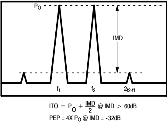
Figure 2. Intermodulation Test
