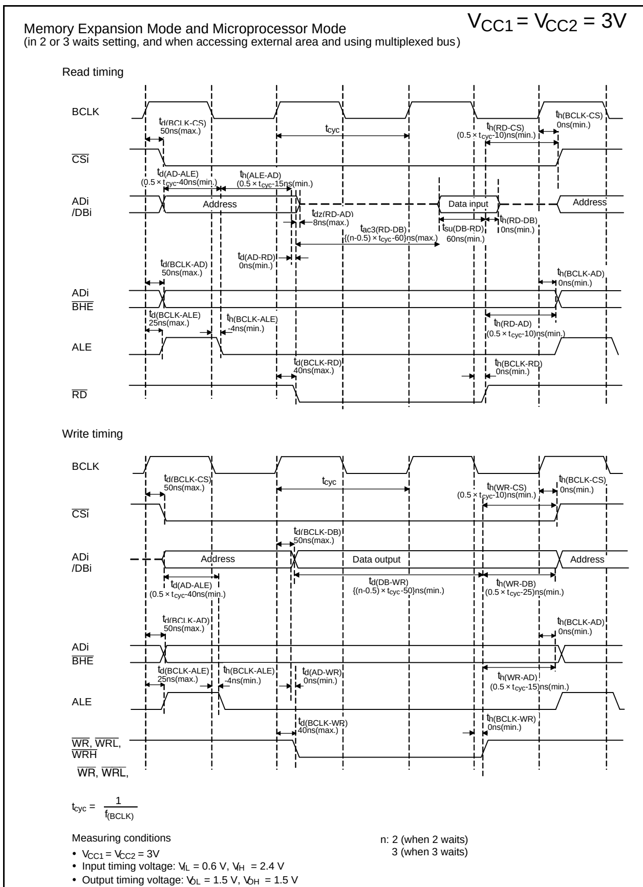
Figure 5.30 Timing Diagram
