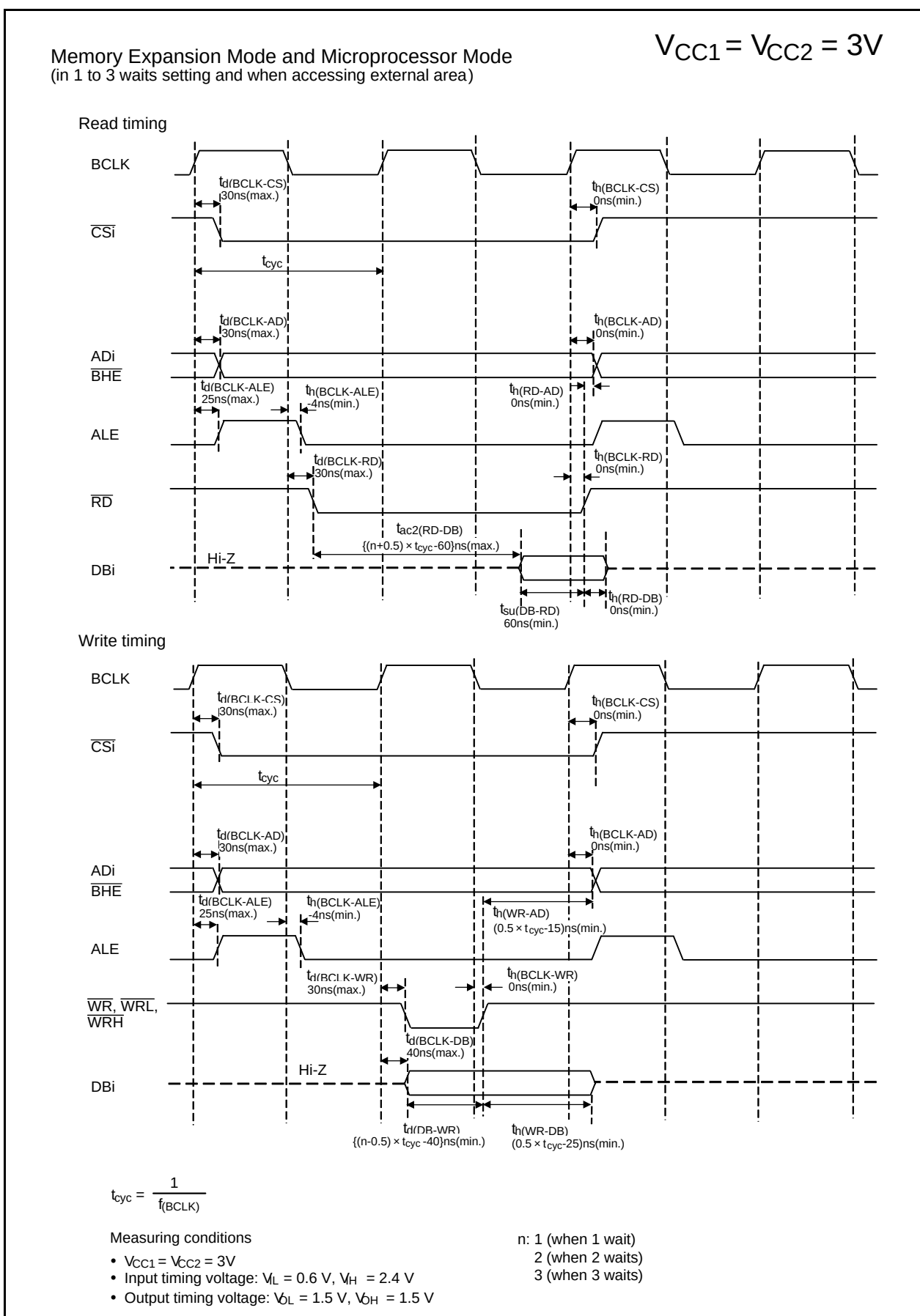
Figure 5.29 Timing Diagram
